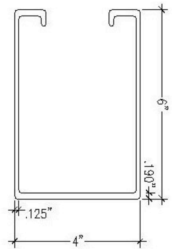
4" x 6" x .125"
